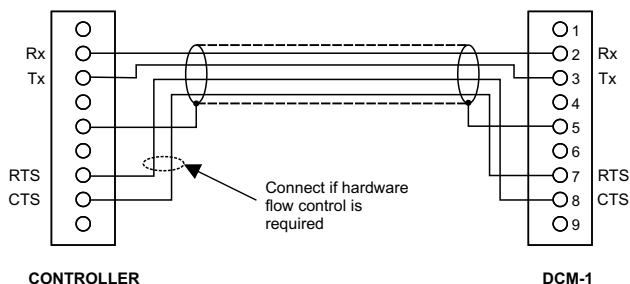
RS232 connection
