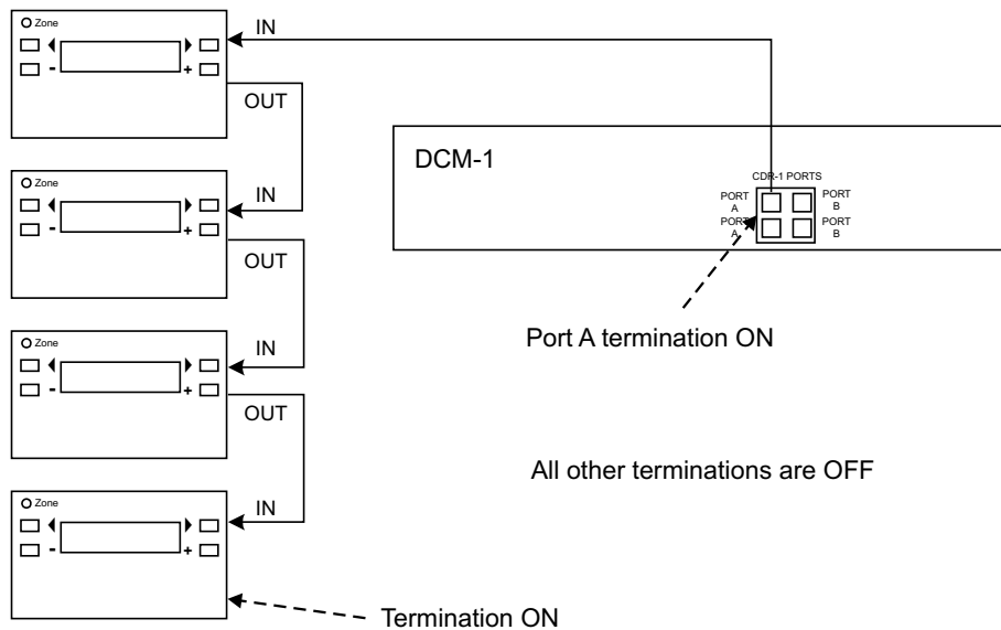
Network diagram 3
