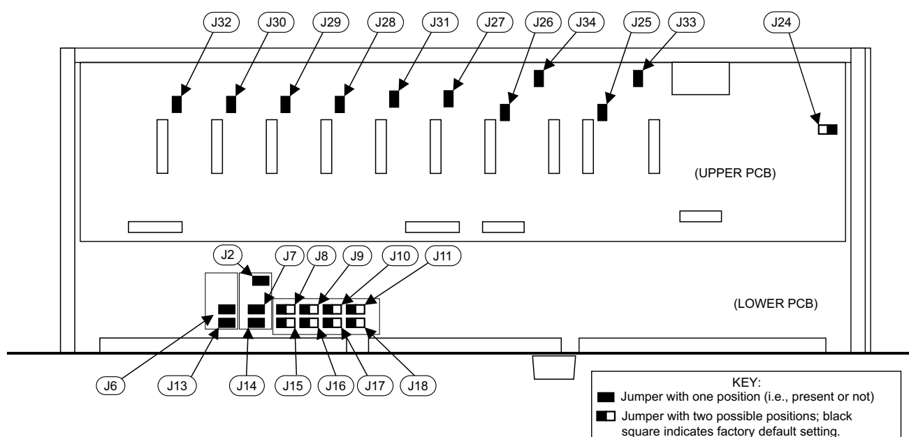
Jumper Locations
