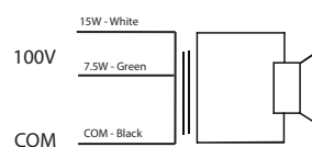
HQ 15EN Circuit diagram
